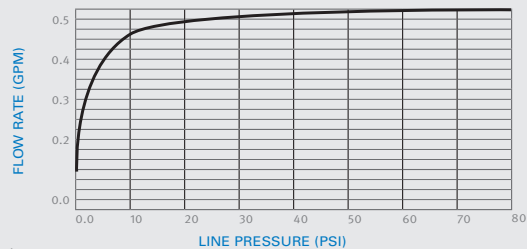
FLOW RATE vs PRESSURE
