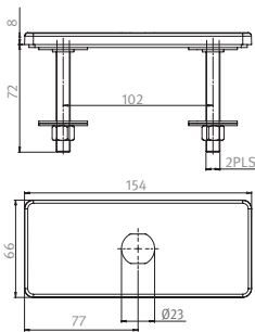
07270288 COVER PLATE 4" ANTI-ROTATION KIT FOR CSABA
