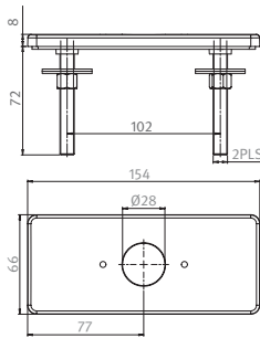
07275005 COVER PLATE 4" ANTI-ROTATION KIT FOR EASY 1000
