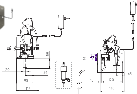
MF BEHIND MIRROR SD/FOAM
