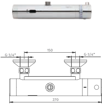
NEPTUNE MEDICAL 1000 T Exposed installation • 610250 NEPTUNE MEDICAL 1000 T , Internal 9V battery
