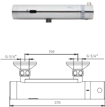
NEPTUNE MEDICAL 1000 T BOTTOM OUTLET Exposed installation Bottom outlet • 610255 NEPTUNE MEDICAL 1000 T BOTTOM OUTLET , Internal 9V battery
