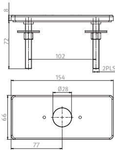
07270290 COVER PLATE 4" ANTI-ROTATION KIT FOR CLASSIC CS
