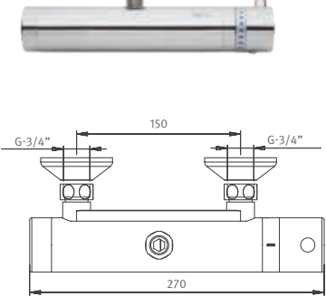
TOUCH SH 1000 T Exposed installation • 610710 TOUCH SH 1000 T , Internal 9V battery
