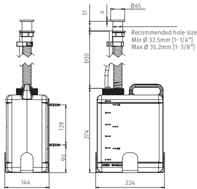
• 07220090 Top-Filling Multifeed Kit
