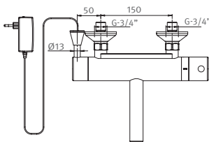
MEDICAL 1000 T Exposed installation Body integrated spout • 314600 MEDICAL 1000 TE , 9V Transformer
