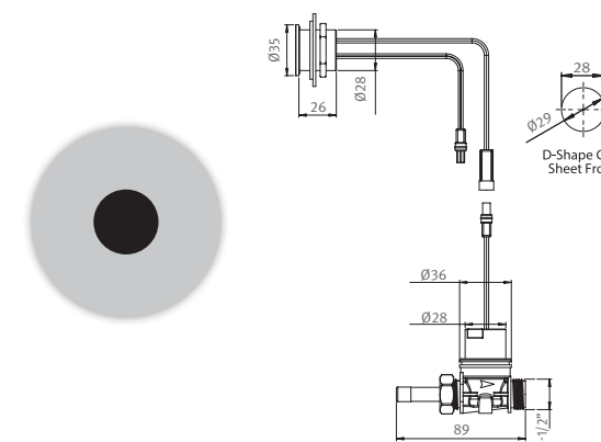
Prox Kit with detachable body for faucet
