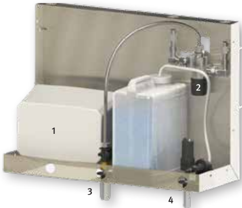
Complete system including high-speed hand dryer (1), thermostatic mixing valve (2), touch-free faucet (3) liquid soap dispenser (4)
