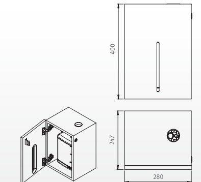
• 07220096 Below Deck Multifeed Kit
