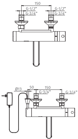
APOLLO MEDICAL Exposed installation Swivel spout
