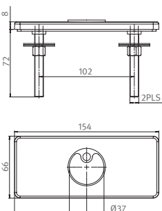
07270291 COVER PLATE 4" ANTI-ROTATION KIT FOR TRENDY/EXTREME
