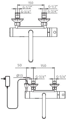
APOLLO MEDICAL F Exposed installation Gooseneck spout
