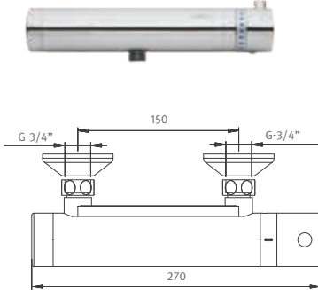
TOUCH SH 1000 T BOTTOM OUTLET Exposed installation Bottom outlet • 610700 TOUCH SH 1000 T BOTTOM OUTLET , Internal 9V battery
